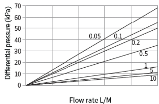
Differential pressure vs. Flow rate (10" PF3/HPF3) (— 0.05=0.05µm)
